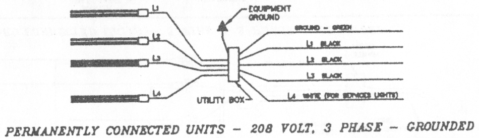
PERMANENTLY CONNECTED UNITS - 208 & 236 VOLT, 1 PHASE - GROUNDED
