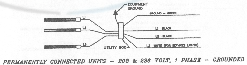
PERMANENTLY CONNECTED UNITS - 115 VOLT, 1 PHASE - GROUNDED
