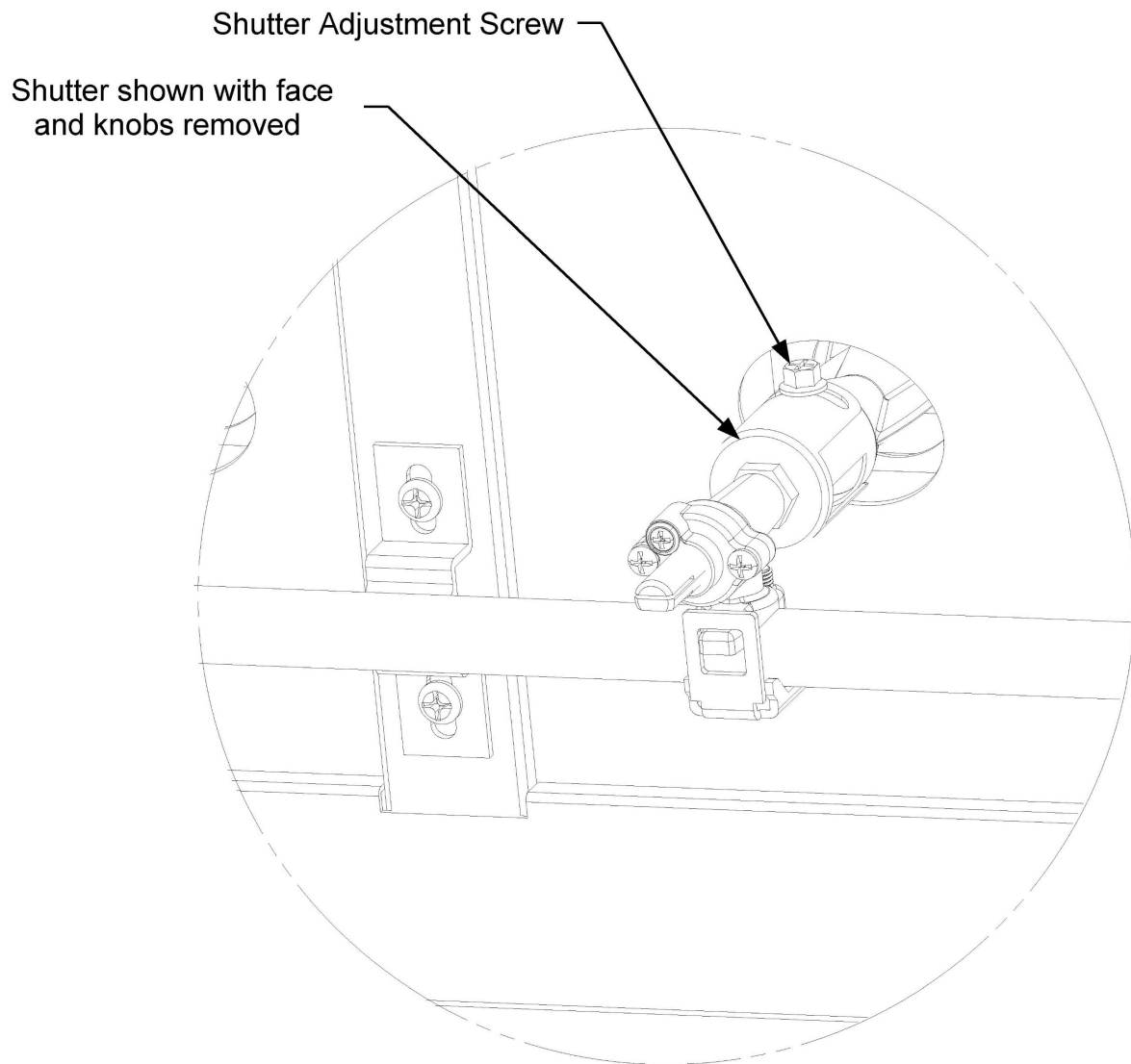
FIGURE 22. SHUTTER ADJUSTMENT
