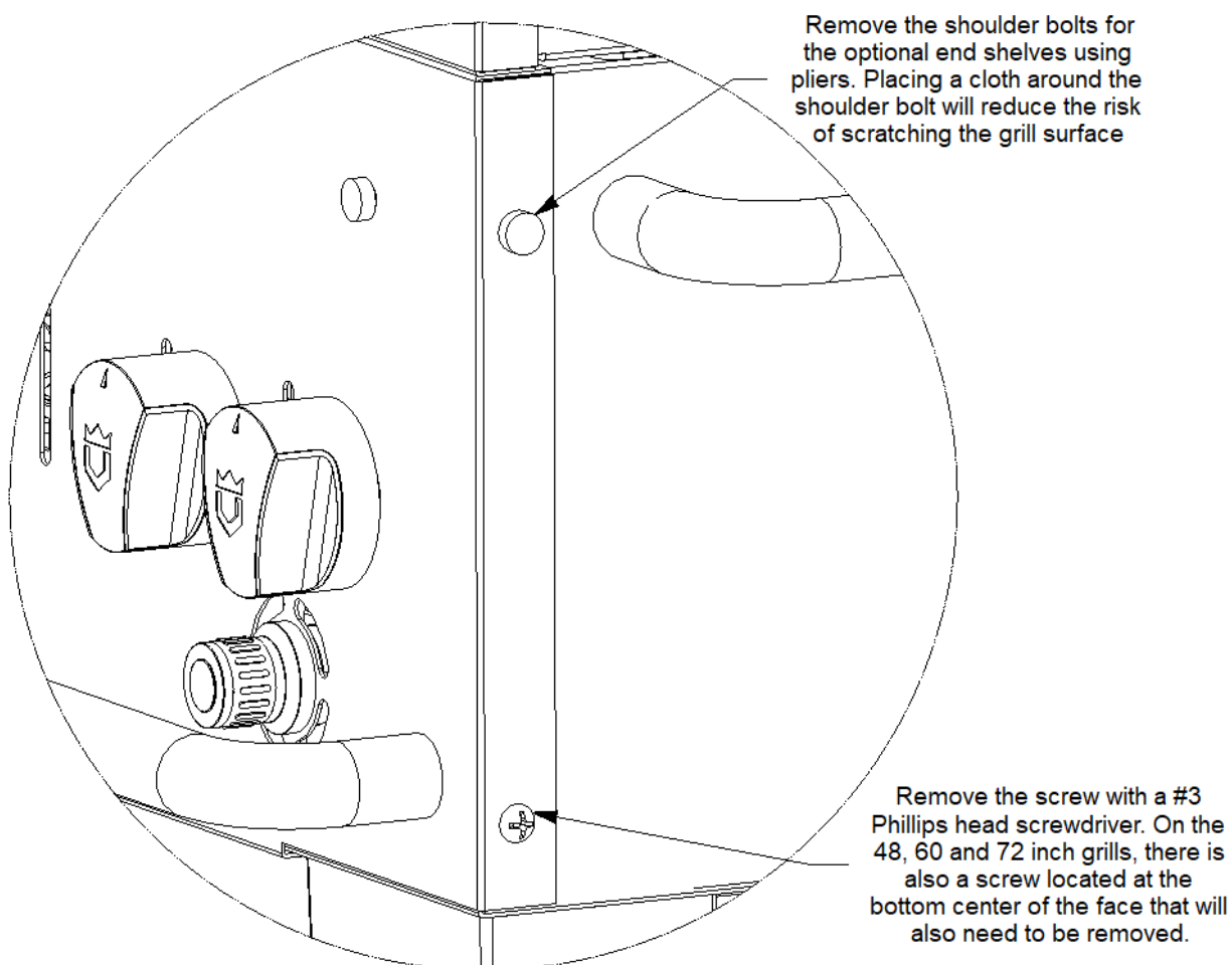
FIGURE 19. FACE REMOVAL
