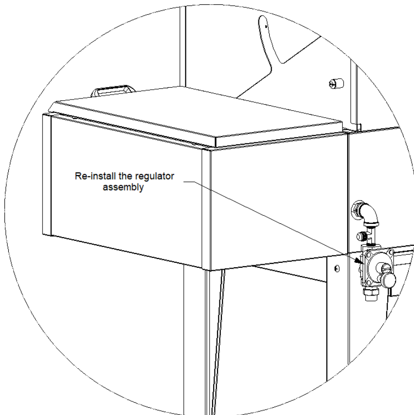
FIGURE 12. RE-INSTALLATION OF REGULATOR FOR SB-MCB
