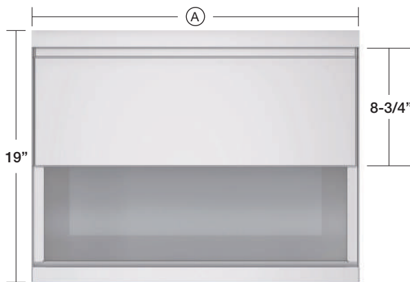
TOP VIEW OF KR19 ICE BIN WITH FULL SLIDING COVER OPEN
