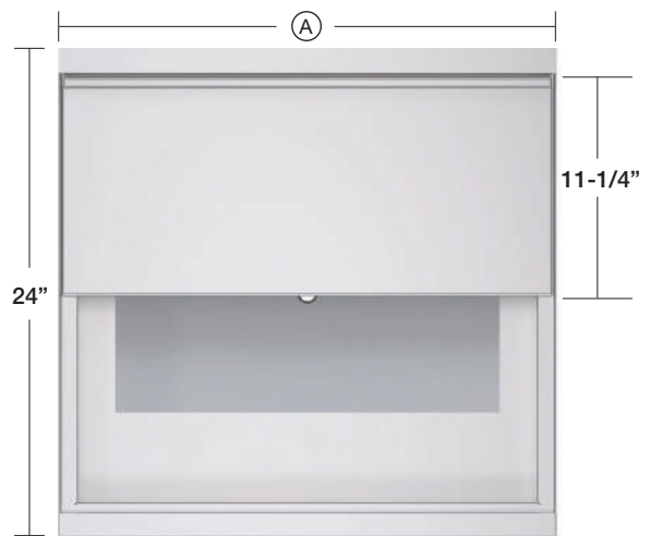
TOP VIEW OF KR24 ICE BIN WITH FULL SLIDING COVER OPEN
