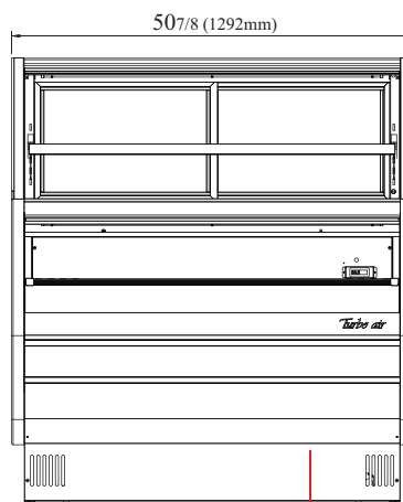
FRONT VIEW ↓ Power Cord (Back of the product)
